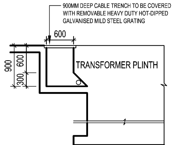
SECTION Z - Z
