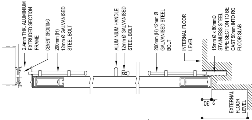
TYPICAL SECTION THROUGH ALUM FLUSHED DOOR SCALE: 1/1.5
