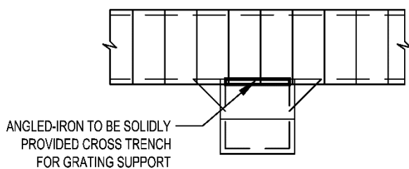
DETAIL AT T- TRENCH
