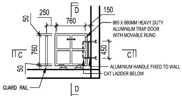
PLAN OF ALUMINIUM TRAP DOOR AND CATLADDER
